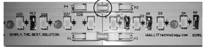
Short connector supplied to join boards together
