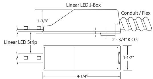
Optional Conduit Feed Adaptor DL-CFB-5600
