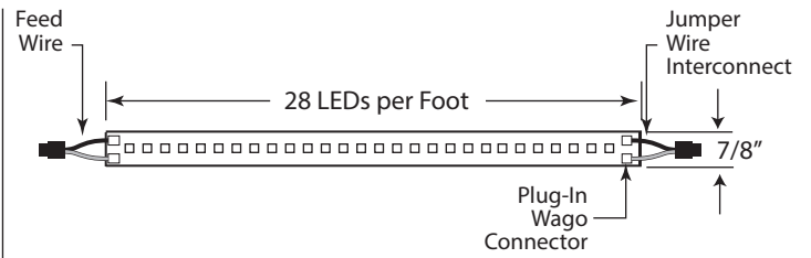
Short connector supplied to join boards together
